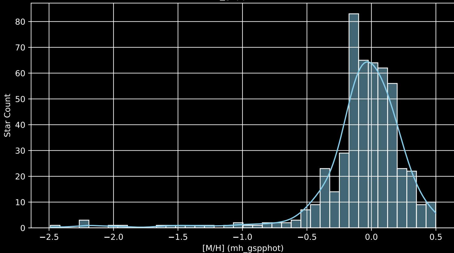
APOGEE DR17 Field: [NGC6791_btx [M/H] (mh_gspphot) (n= 502)
