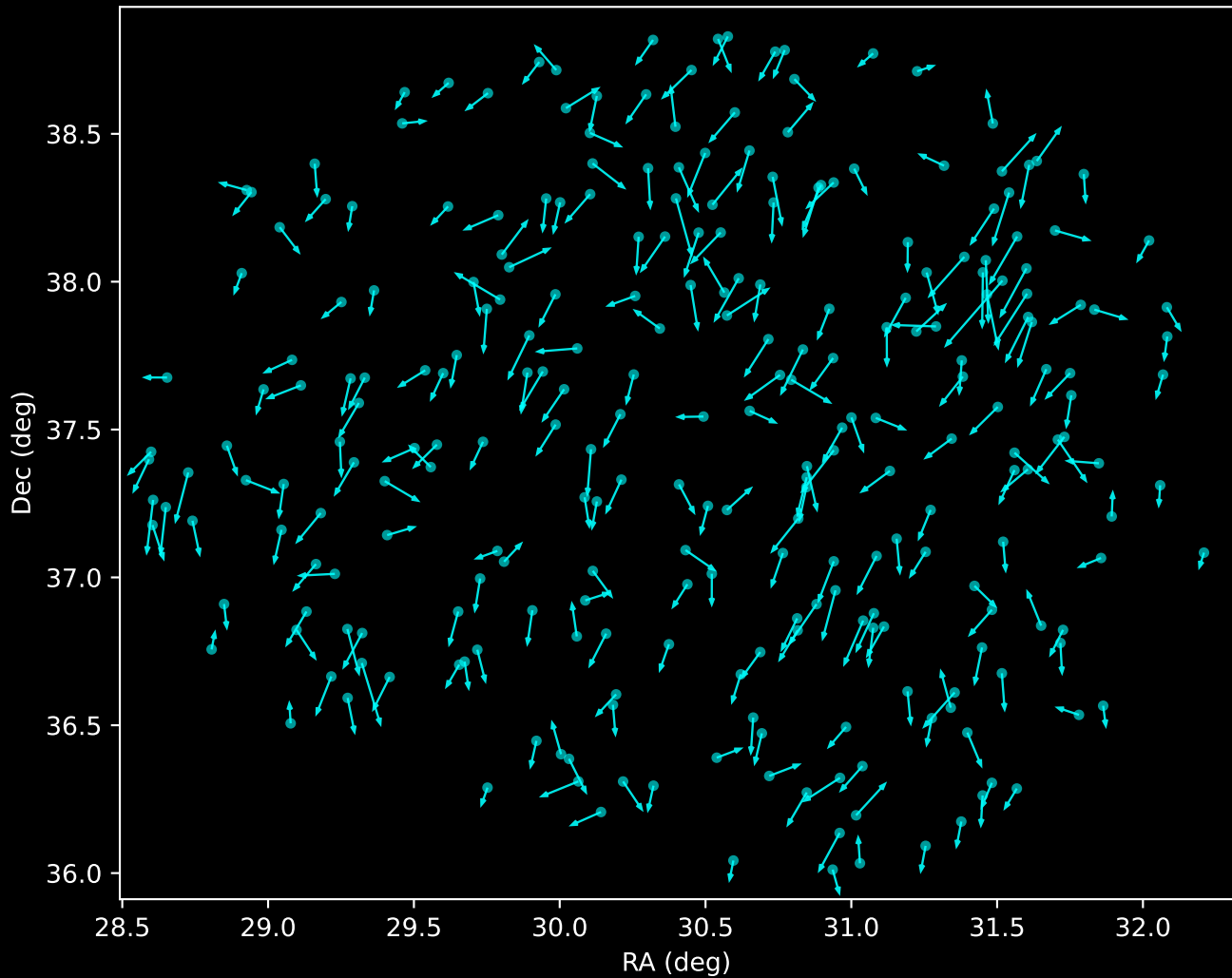
APOGEE DR17 Noise Stream Proper Motion Vectors (n=264)
