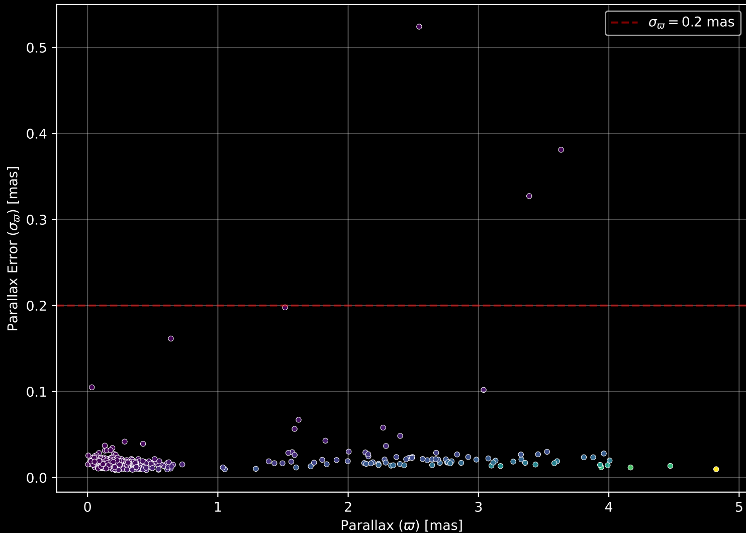
APOGEE DR17 Field: [NGC6791_btx] Parallax Quality (n= 507)
