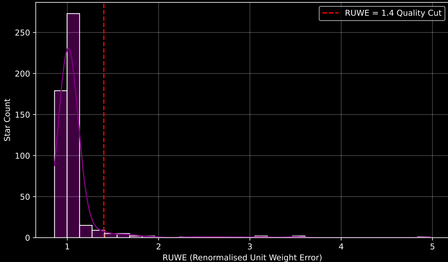
GAPOGEE DR17 Field [NGC6791_btx] RUWE Distribution (n= 500)
