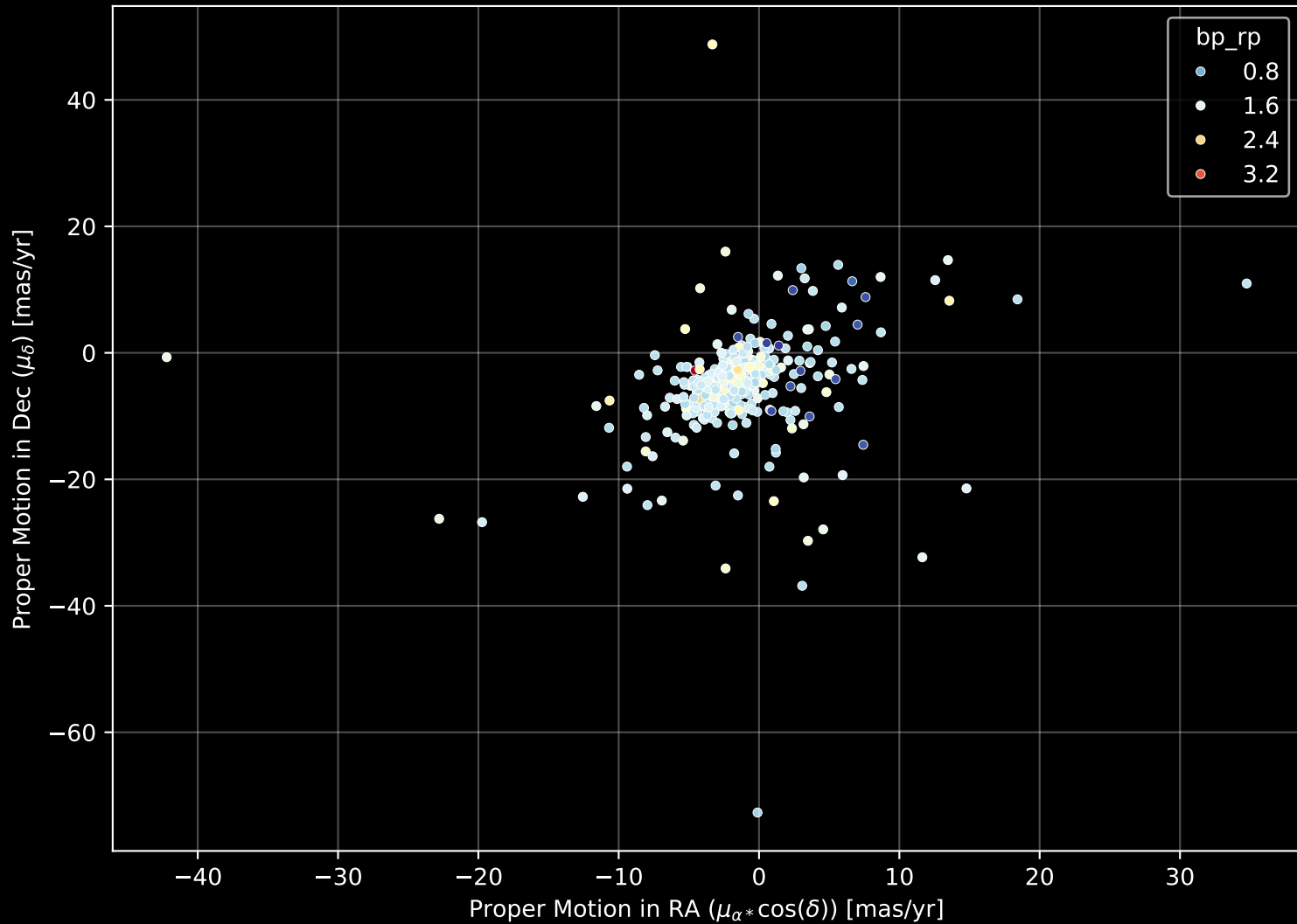
APOGEE DR17 Field: [NGC6791_btx] Proper Motion Diagram (n= 507)
