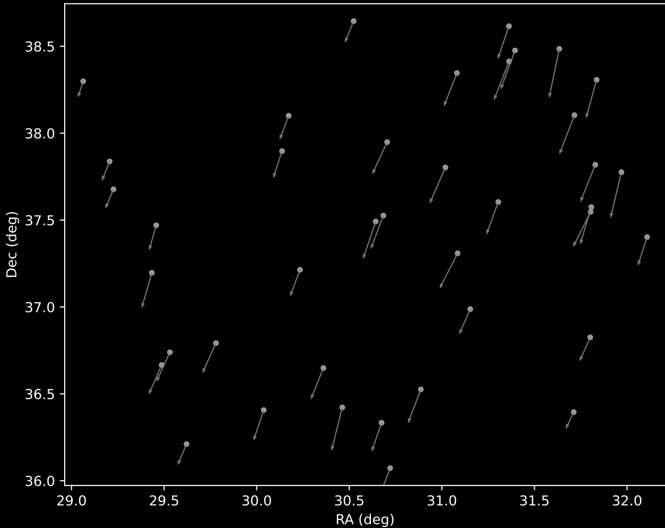
APOGEE DR17 Cluster 14 Proper Motion Vectors (n=40)
