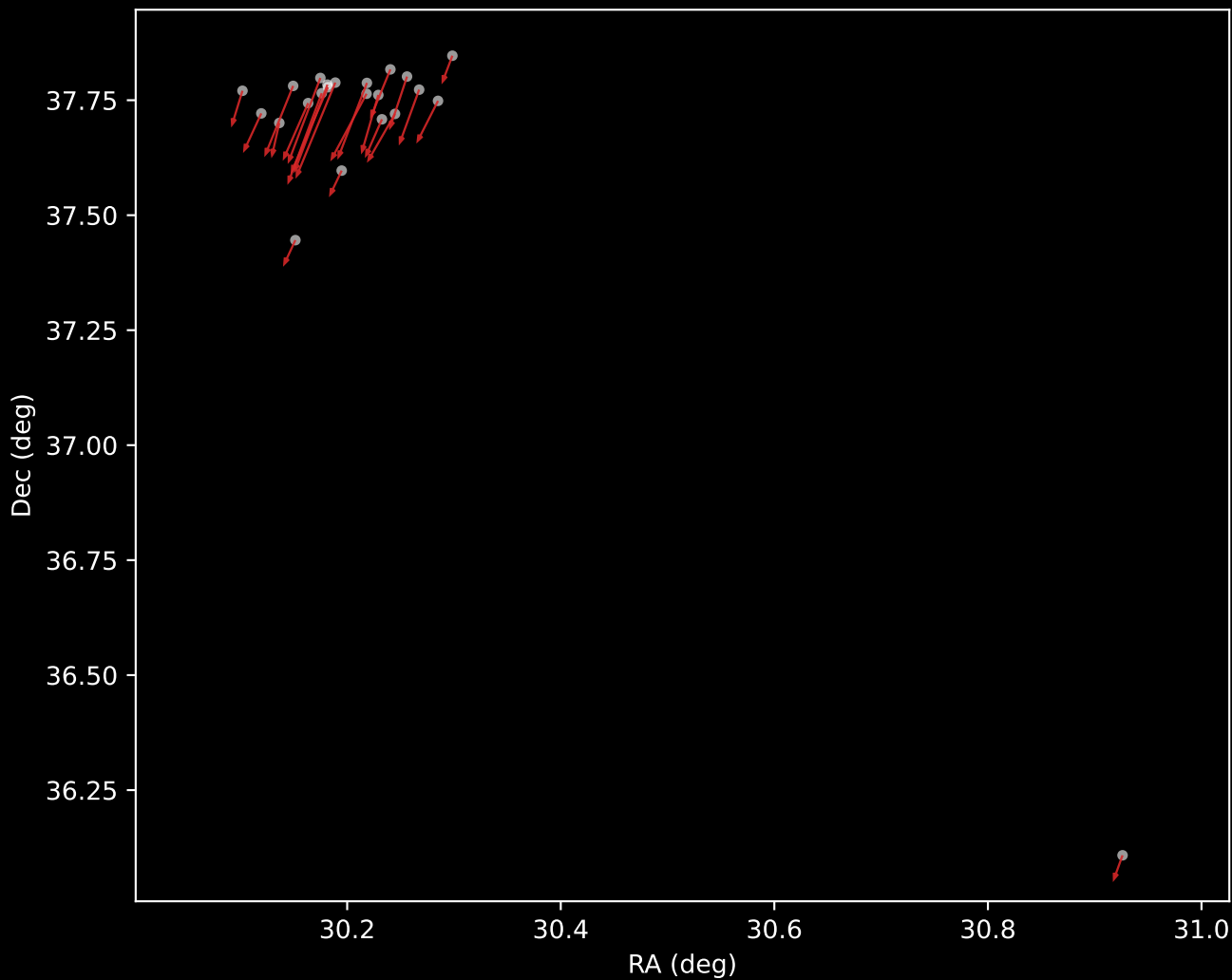
APOGEE DR17 Cluster 6 Proper Motion Vectors (n=23)
