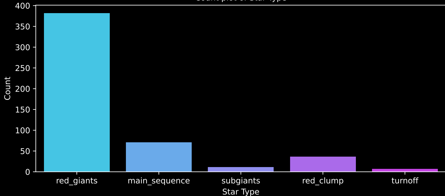
APOGEE DR17 Field: [NGC6791_btx] Count plot of Star Type
