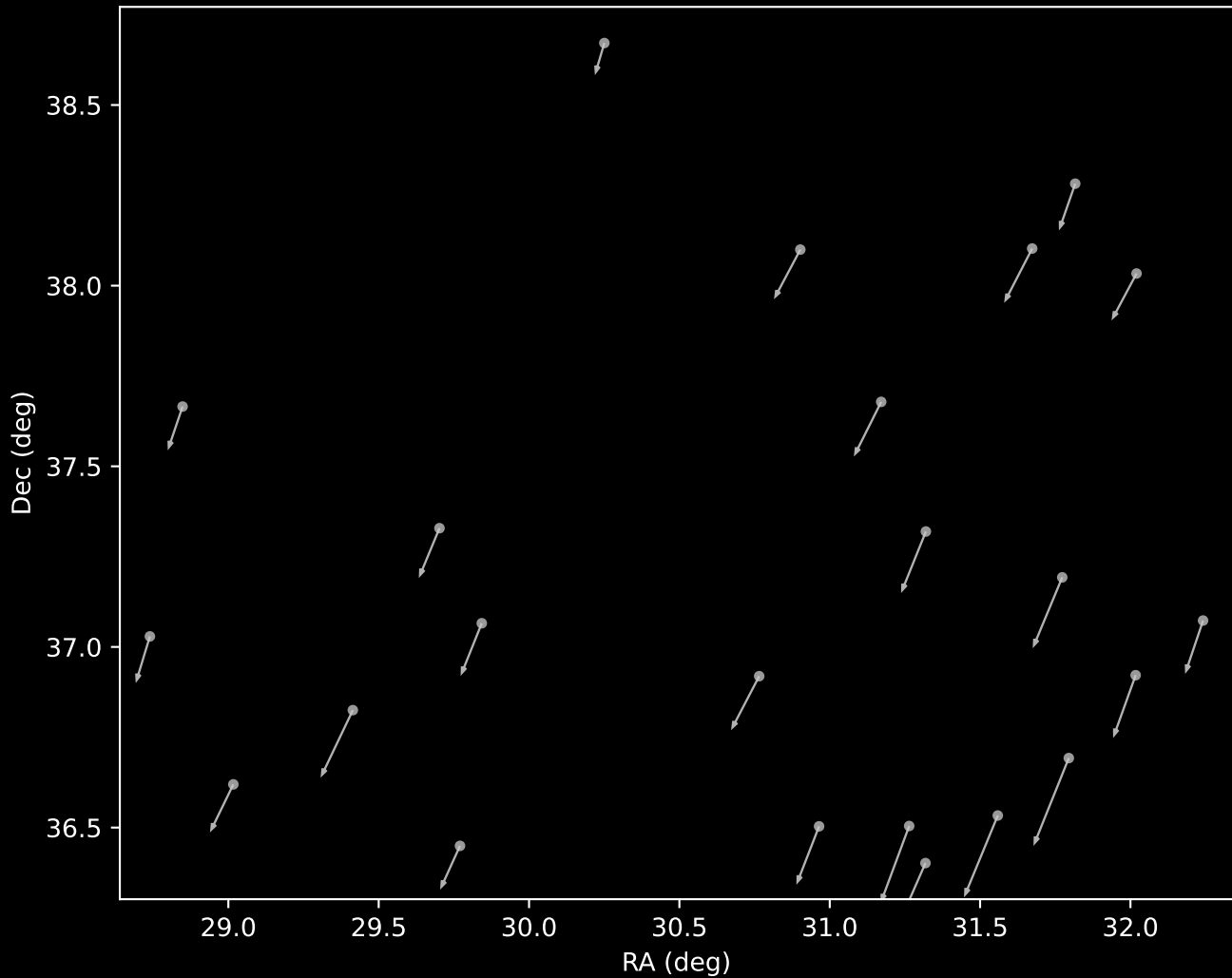
APOGEE DR17 Cluster 15 Proper Motion Vectors (n=23)
