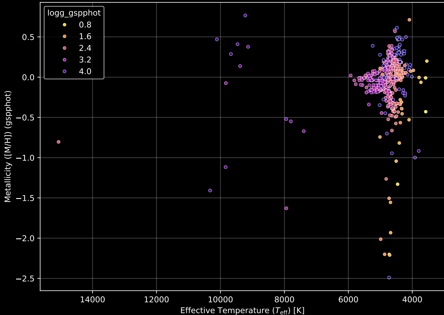
APOGEE DR17 Field: [NGC6791_btx] Stellar Population Parameters (n= 507)
